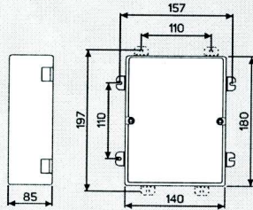
Fig.1 - ENCOMBREMENT (mm):
