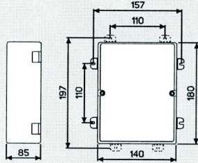
Fig.1 - DIMENSIONS (mm):
